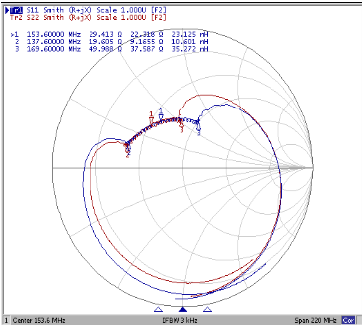
Smith Chart
