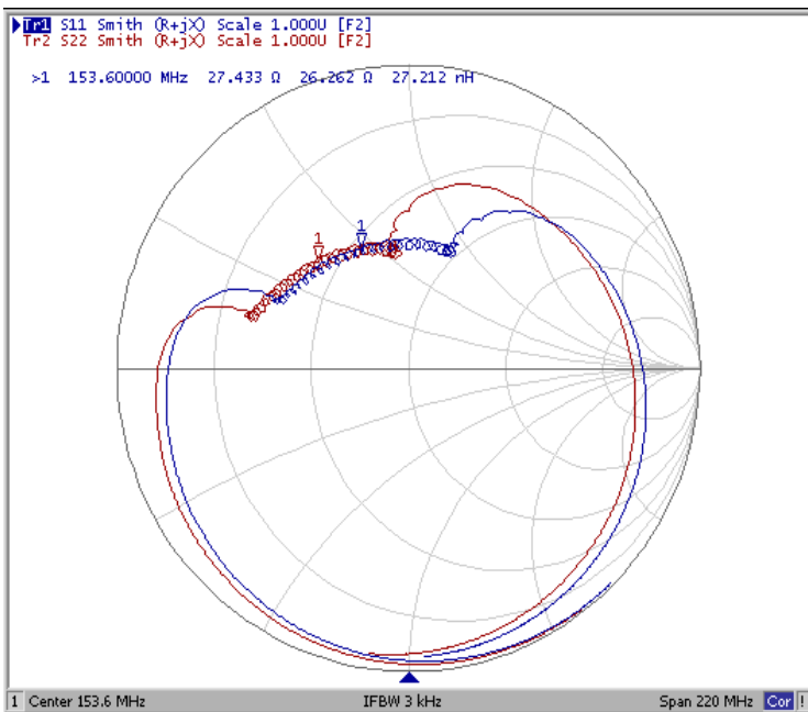
Smith Chart
