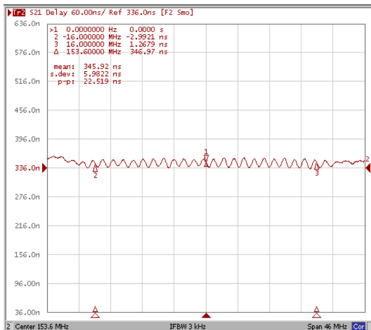
Group Delay Variation Fo±16.00MHz
