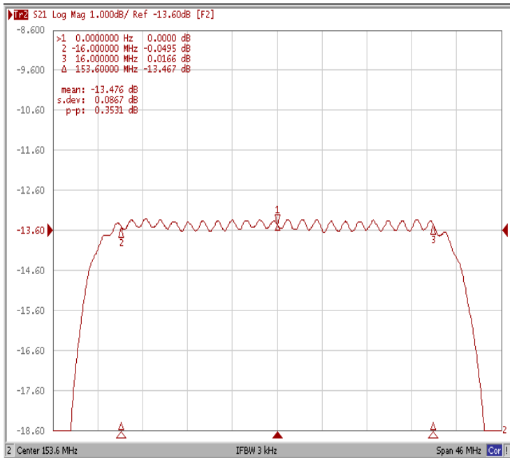
Ripple Variation Fo±16.00MHz
